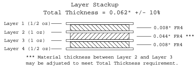
(a) Total Thickness 0.062"
