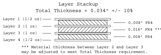
(b) Total Thickness 0.8mm
