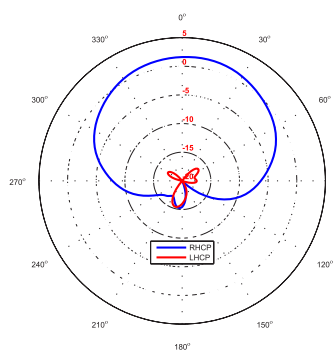
GLONASS RHCP Gain
